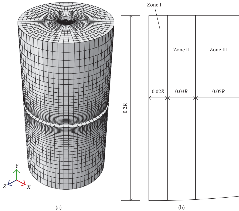
FIGURE 1: 3D finite element mesh for identical spheres. (a) 3D FE mesh for two identical spheres in contact. (b) Zone partition of the sphere.
