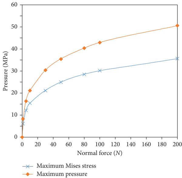
FIGURE 2: Contact pressure versus normal force.
