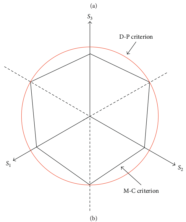
FIGURE 4: Yield surface for the linear D-P criterion versus V-M criterion and the linear D-P criterion versus M-C criterion: (a) D-P versus Mises criterion in the I_1 - \sqrt{J_2} plane; (b) D-P versus M-C criterion in the \pi plane.
